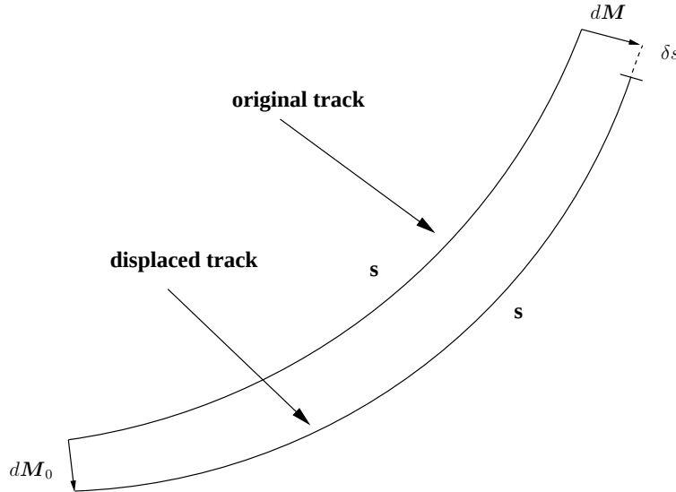
Figure 1: A track and the displaced track due to a variation d\mathbf{M}_0 are shown. In the error propagation the change \delta s of the path length has to be taken into account. In this specific case d\mathbf{M} is understood to be perpendicular to the track (see also Eq. (21)).
